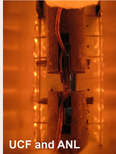
Fiber optic probe coupled with electromechanical testing system at UCF for Piezo-spectroscopic studies
