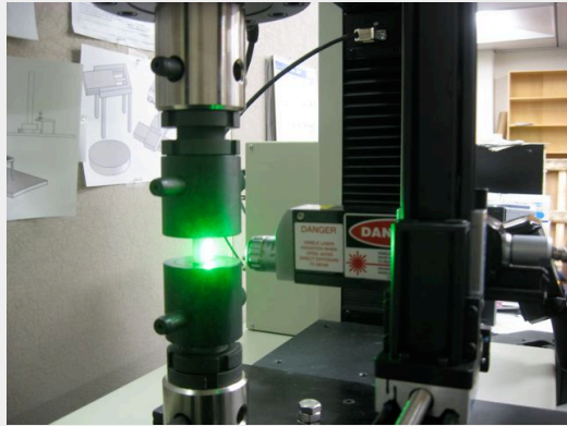
Fiber optic probe coupled with electromechanical testing system at UCF for Piezo-spectroscopic studies
