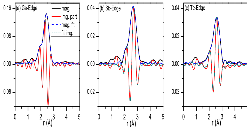
Atomic structure of electrodeposited a-Ge 2 Sb 2 Te 5 measured by extended X-ray absorption fine structure
