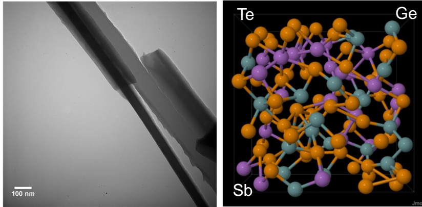
Left: TEM image of amorphous phase-change nanowire Right: Simulated atomic structure of amorphous Ge 2 Sb 2 Te 5
