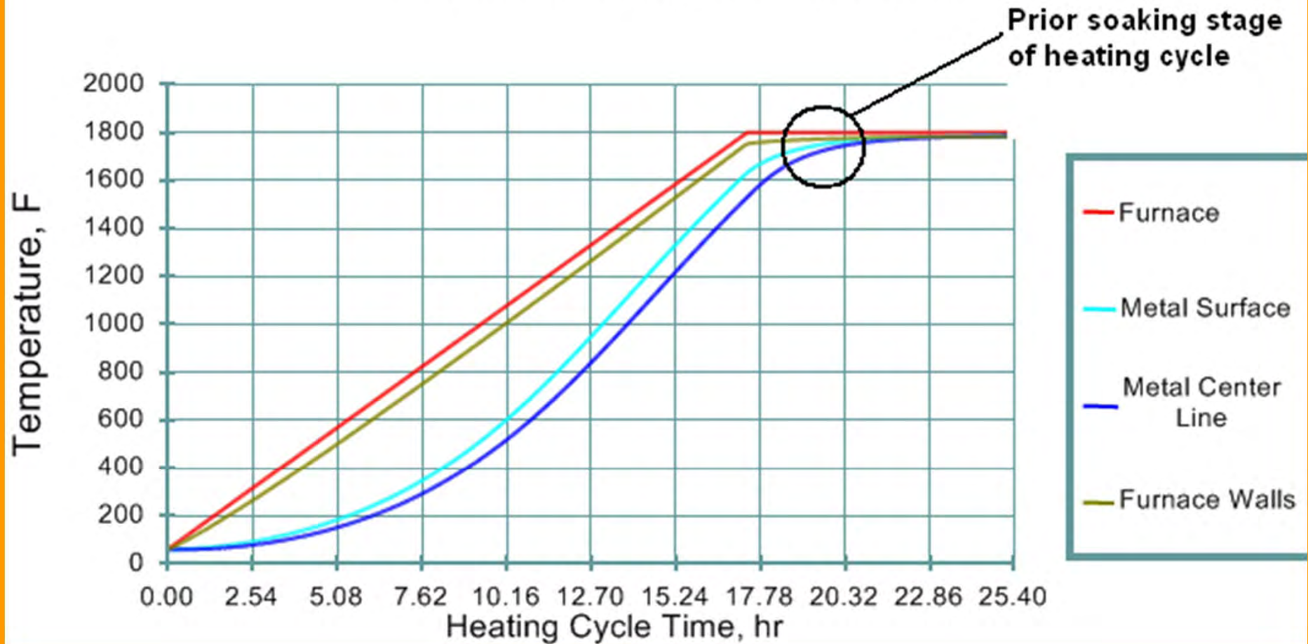
Furnace Temperature Profile
