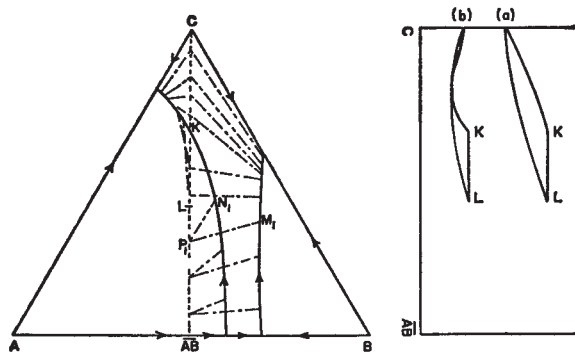
FIG. XXIV.—Ternary system containing a binary compound unstable at its melting point which forms a series of solid solutions with the third component.
