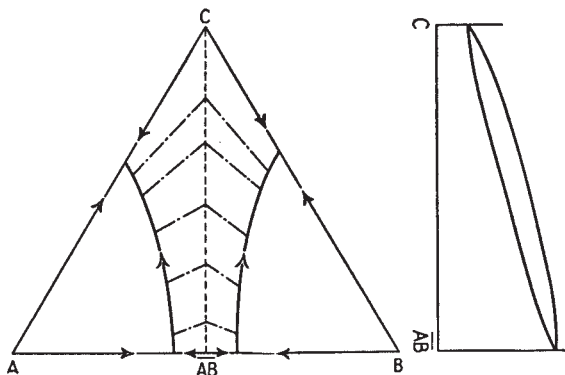
FIG. XXIII.—Ternary system containing a binary compound stable at its melting point which forms a complete series of solid solutions with the third component.
