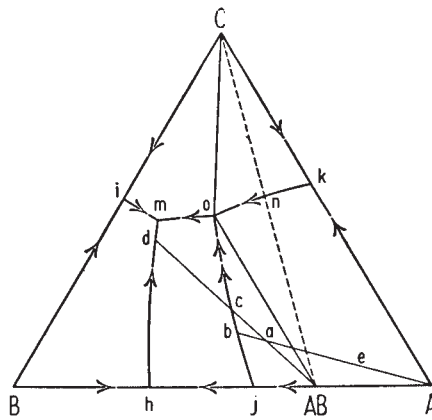
FIG. XVII.—Ternary system containing a binary compound unstable at its melting point. O. Andersen, Am. J. Sci. , 4th Ser., 39, 433 (1915).
