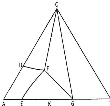
FIG. XXV.—Determination of the position of the three-phase boundary, F-G .
