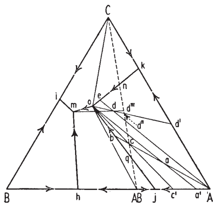
FIG. XVI.—Ternary system with a binary compound which does not form a binary system with the third component. O. Andersen, Am. J. Sci. , 4th Ser., 39, 431 (1915).
